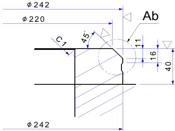
DETAIL Aa (1:2)
